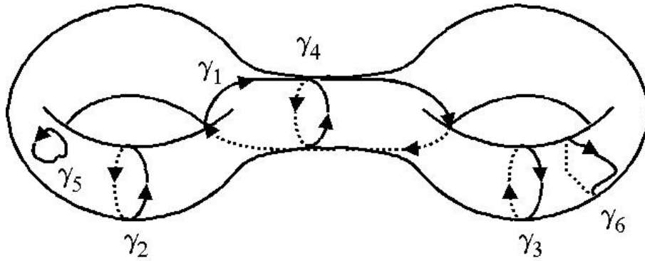
Figure 1.20. A closed surface with two handles marked by several different closed 1–dimensional paths
