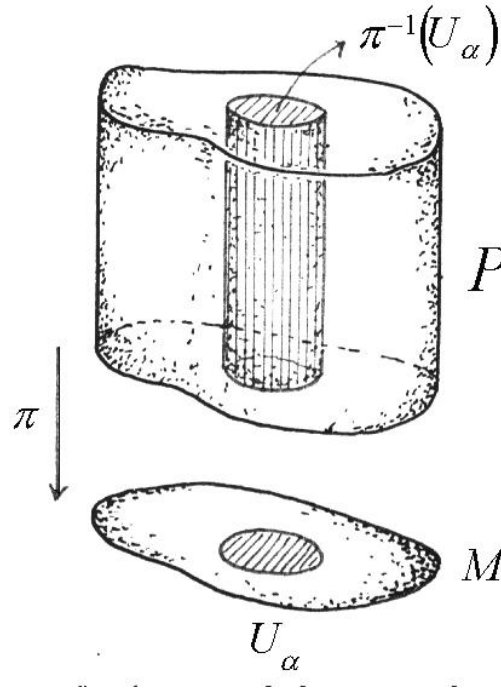
Figure 1.13. A fibre–bundle is locally trivial
