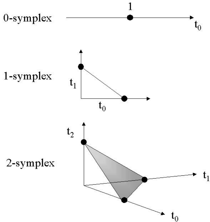
Figure 1.25. The standard p -simplices for p = 0, 1, 2
