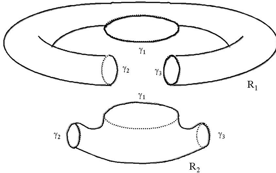
Figure 1.22. The sum of the three paths \gamma_1, \gamma_2, \gamma_3 is homologically trivial, namely \gamma_2 + \gamma_3 is homologous to -\gamma_1
