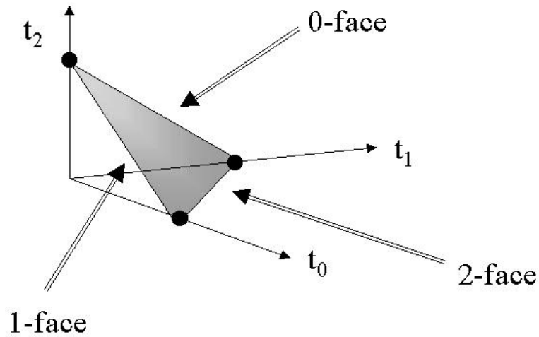
Figure 1.27. The faces of the standard 2-simplex
