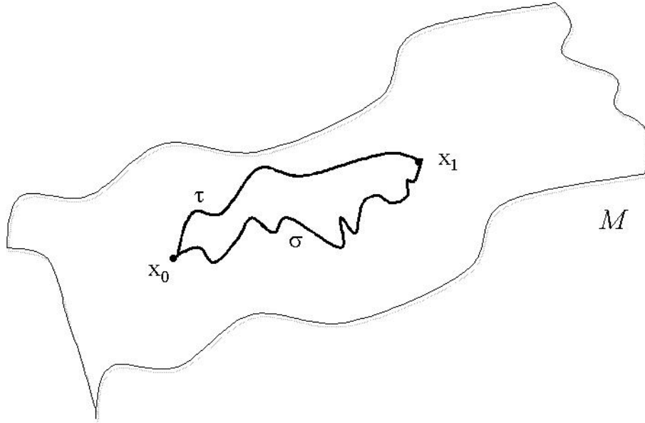
Figure 1.23. Two paths with coinciding extrema
