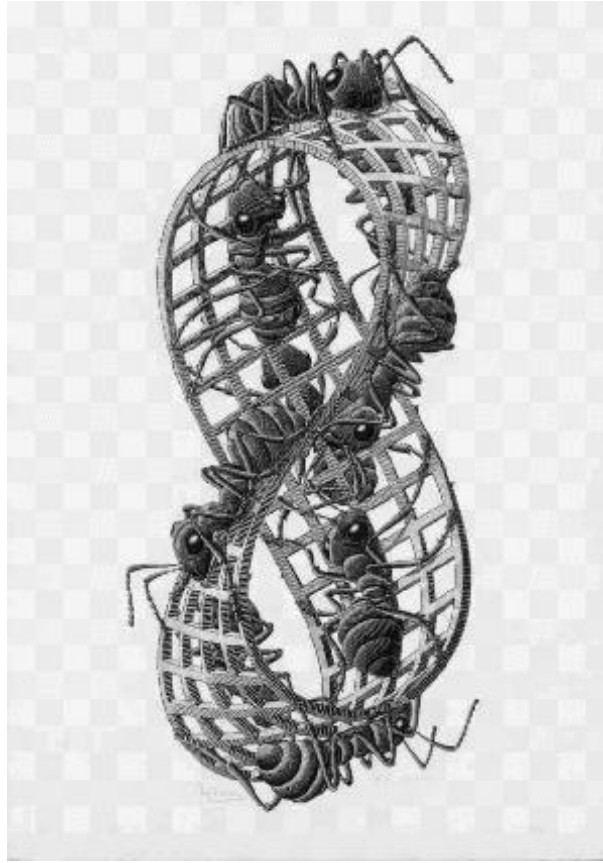
Figure 1.12. Escher’s ant crawling on a Möbius strip is a pedagogical example of a fibre–bundle
