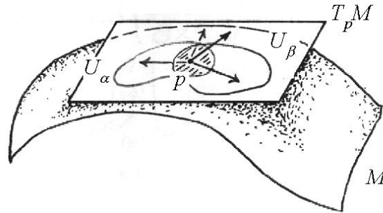
Figure 1.17. Two local charts of the base manifold \mathcal{M} yield two local trivializations of the tangent bundle T\mathcal{M}
