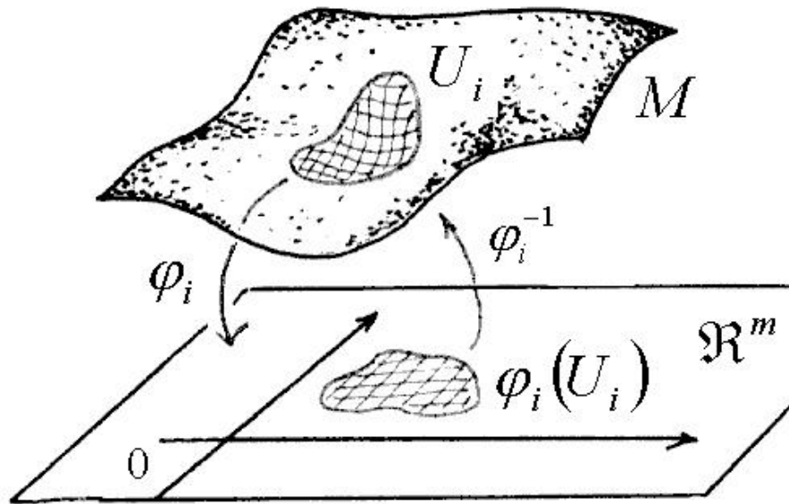
Figure 1.1. An open chart is a homeomorphism of an open subset U_i of the manifold \mathcal{M} onto an open subset of \mathbb{R}^m
