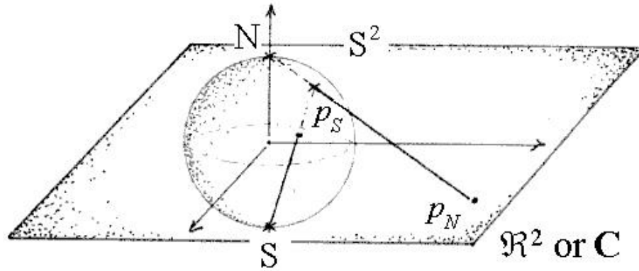
Figure 1.3. Stereographic projection of the two sphere
