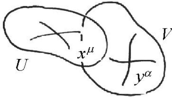
Figure 1.11. Two coordinate patches
