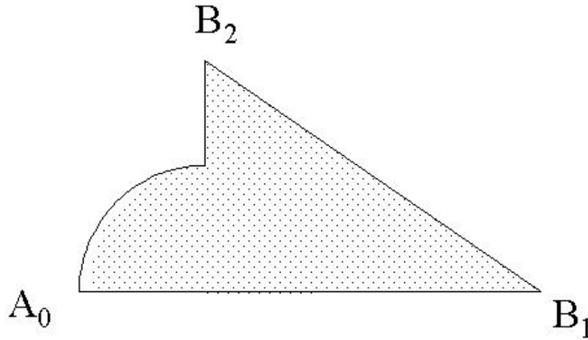
Figure 1.29. Geometrically the chain S_1^{(2)} + S_2^{(2)} is the union of the two simplexes S_1^{(2)} \cup S_2^{(2)}
