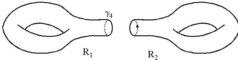
Figure 1.21. When we cut a surface along a path that is a boundary, namely it is homologically trivial, the surface splits into two separate parts
