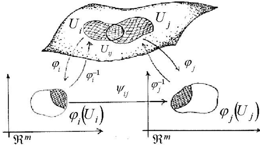
Figure 1.2. A transition function between two open charts is a differentiable map from an open subset of \mathbb{R}^m to another open subset of the same.
