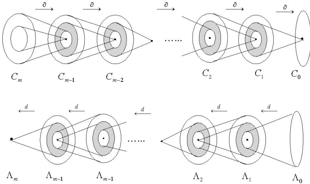
Figure 1.31. Homology versus cohomology groups.
