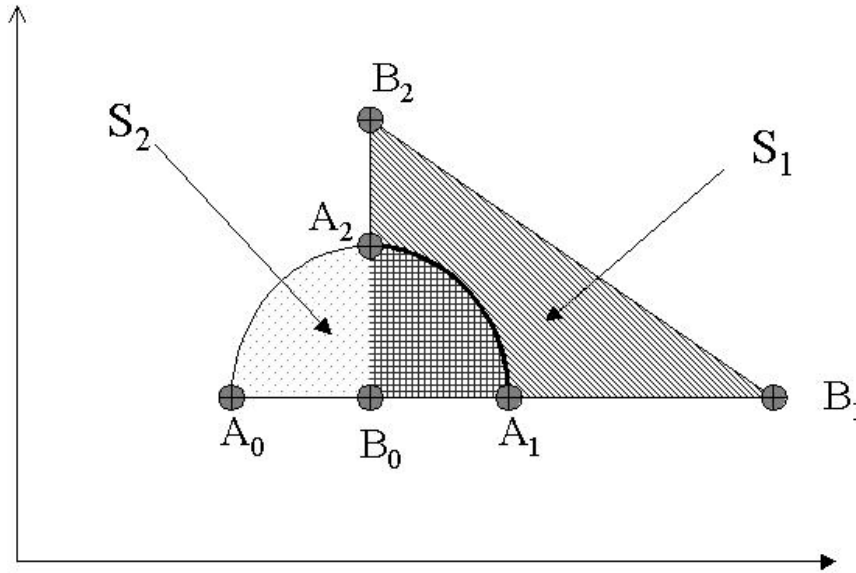
Figure 1.28. S_1^{(2)} and S_2^{(2)} are two distinct 2-simplexes, namely two triangles with vertices respectively given by (A_0, A_1, A_2) and (B_0, B_1, B_2) . The 2-simplex S_3^{(2)} with vertices B_0, A_1, A_2 is the intersection of the other two S_3^{(2)} = S_1^{(2)} \cap S_2^{(2)}
