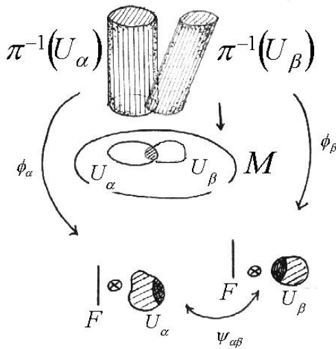
Figure 1.14. Transition function between two local trivializations of a fibre-bundle
