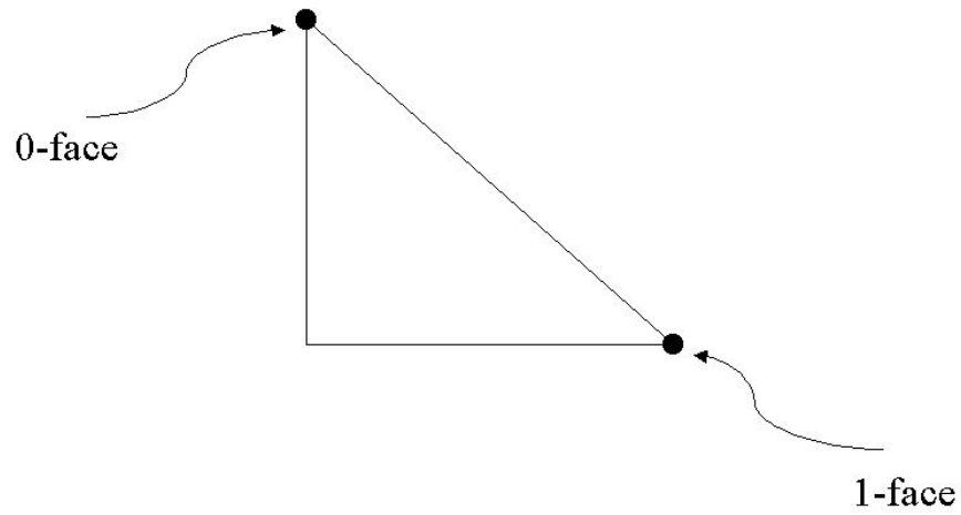
Figure 1.26. The faces of the standard 1-simplex
