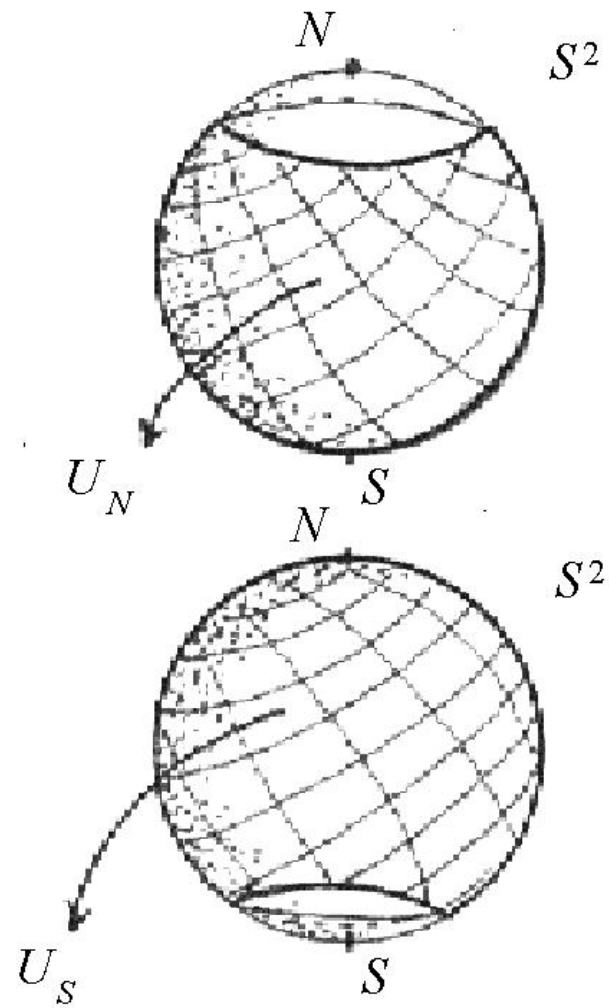
Figure 1.4. The open charts of the North and South Pole
