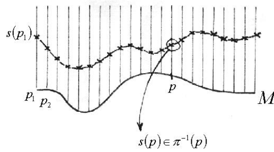
Figure 1.18. A section of a fibre bundle
