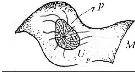
Figure 1.8. In a neighborhood U_p of each point p \in \mathcal{M} we consider the curves that go through p
