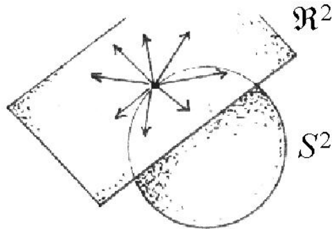
Figure 1.9. The tangent space in a generic point of an \mathbb{S}^2 sphere
