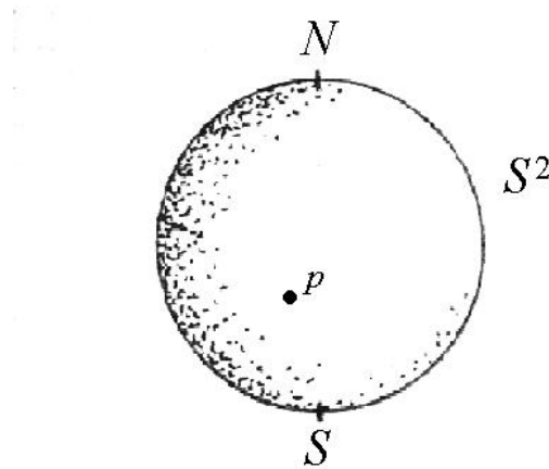
Figure 1.19. A section of a fibre bundle
