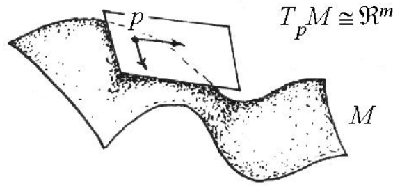
Figure 1.16. The tangent bundle is obtained by gluing together all the tangent spaces
