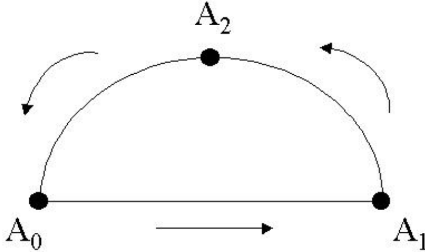
Figure 1.30. The oriented boundary of the S^{(2)} symplex.
