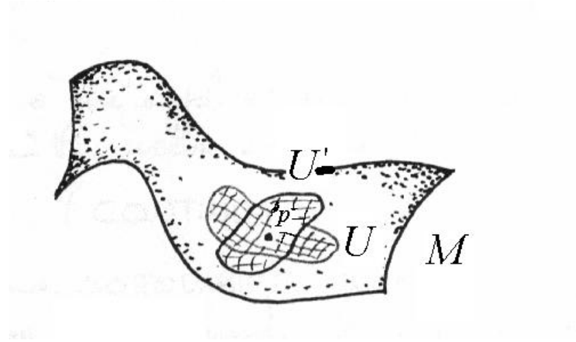
Figure 1.6. A germ of smooth function is the equivalence class of all locally defined function that coincide in some neighborhood of a point p
