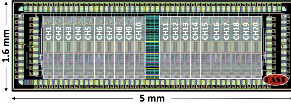
Figure 1: Layout top view of the 1.6 mm \times 5 mm FAST prototype.
