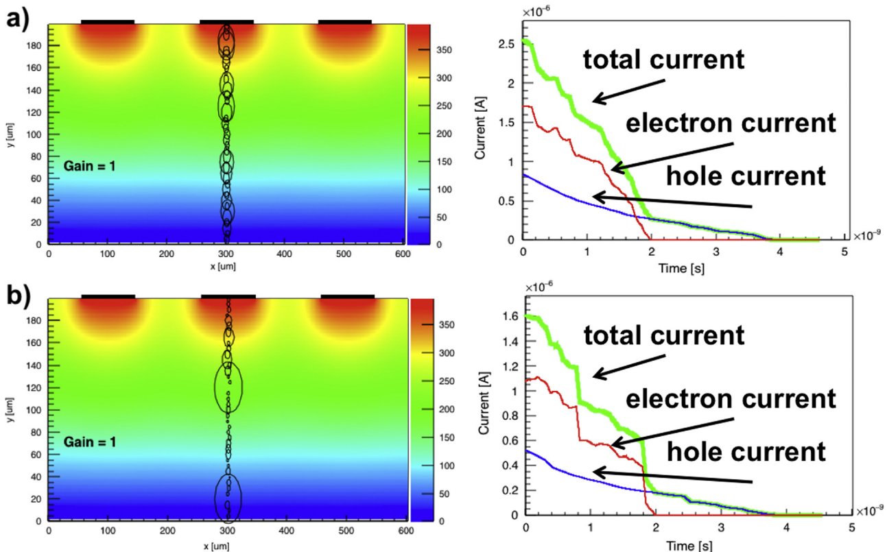
Fig. 1. a) Energy deposits in a silicon detector with gain =1, and (b) the corresponding current signals.
