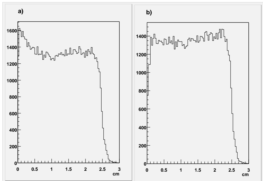
Figure 6: Crossing point of the cosmic ray on the plane of the sense wires. a) constant velocity model, b) cell modeled using GARFIELD.
