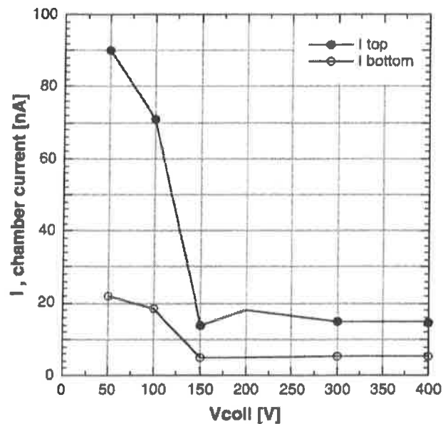
Figure 2.51: Influence of V_{coll} on the chamber current. PC32. HV = 2050 V, 10 000 particles/burst. I_{top} is measured in the half of the chamber crossed by the direct beam. I_{bottom} is the other half.
