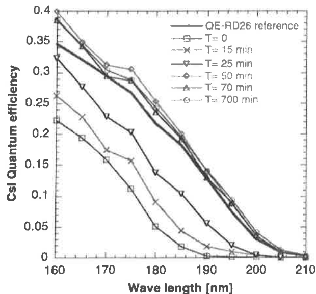
Figure 2.8: Effect of the heating of the CsI sample after evaporation at 60 °C under vacuum. From T = 0 (the end of evaporation), an enhancement of the QE with time is observed. Measurements made at the Weizmann Institute using a CERN PCB substrate.
