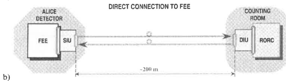
Figure 3.37: (a) DDL logical interface. (b) Direct connection between the front-end electronics on the detector and the DDL.
