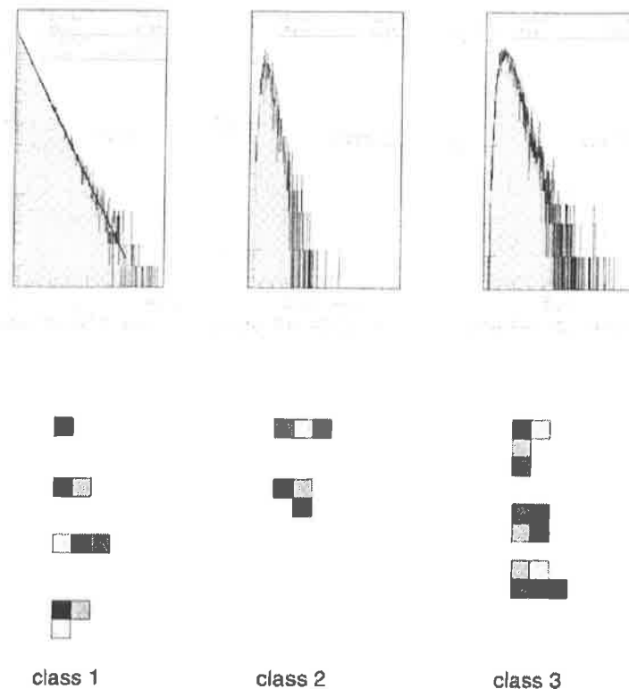
Figure 2.72: (top) The total pulse-height distributions of the three classes of raw clusters and (bottom) the geometrical features for each class (the darker the grey tone, the larger the pad pulse height).
