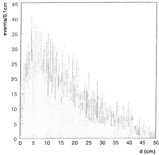
Figure 2.68: The distribution of distances d of track impact points measured on the HMPID cathode plane from the beam line.
