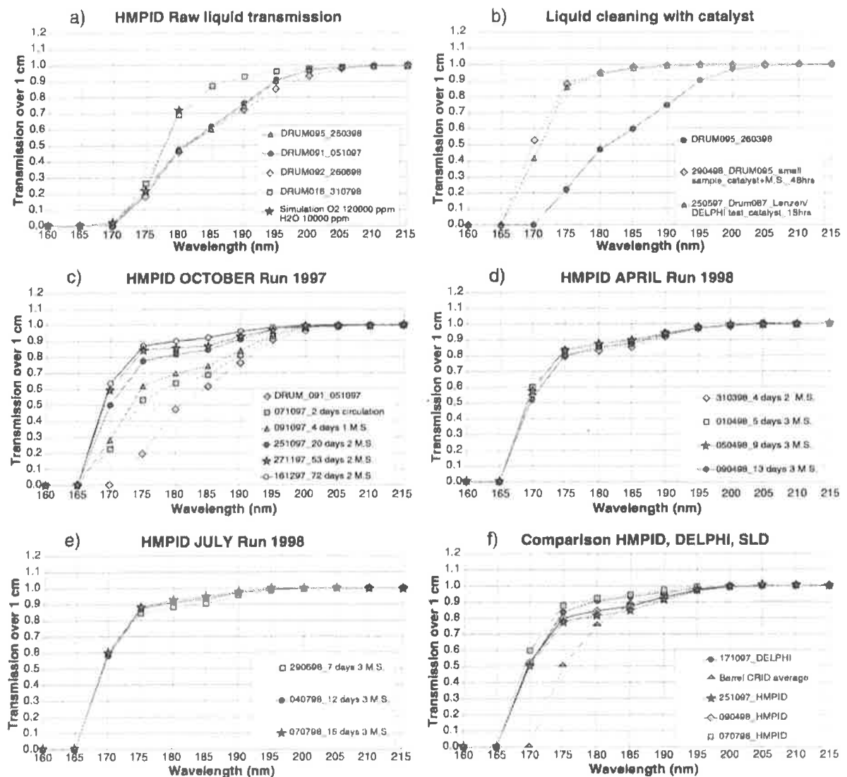
Figure 3.14: Transparency curves for different samples. For details see text.
