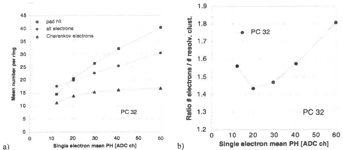
Figure 2.36: Experimental conditions: proto-2, PC32, 10 mm C_6F_{14} radiator, CH_4 , pions 350 GeV/c. a) Plots of the mean number per ring of pad hits ( N_{pad} ), electrons ( N_{tot} ) and Cherenkov electrons ( N_{res} ) as a function of the single-electron mean PH. b) Ratio N_{tot}/N_{res} , number of electrons per cluster. One ADC channel corresponds to 0.17 fC.
