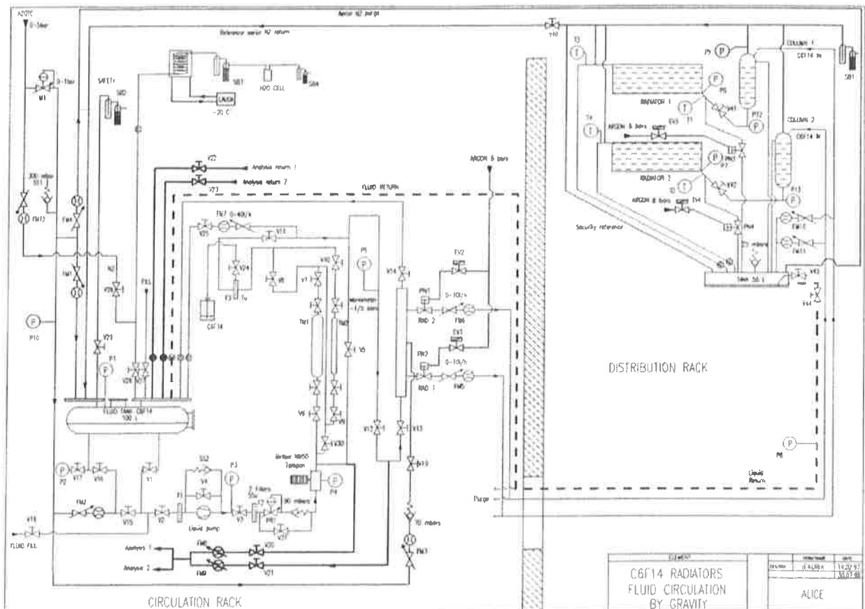
Figure 3.12: Circuit diagram of the recirculation system.
