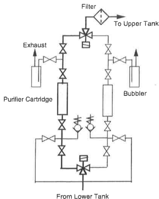
Figure 3.45: Purifier unit.
