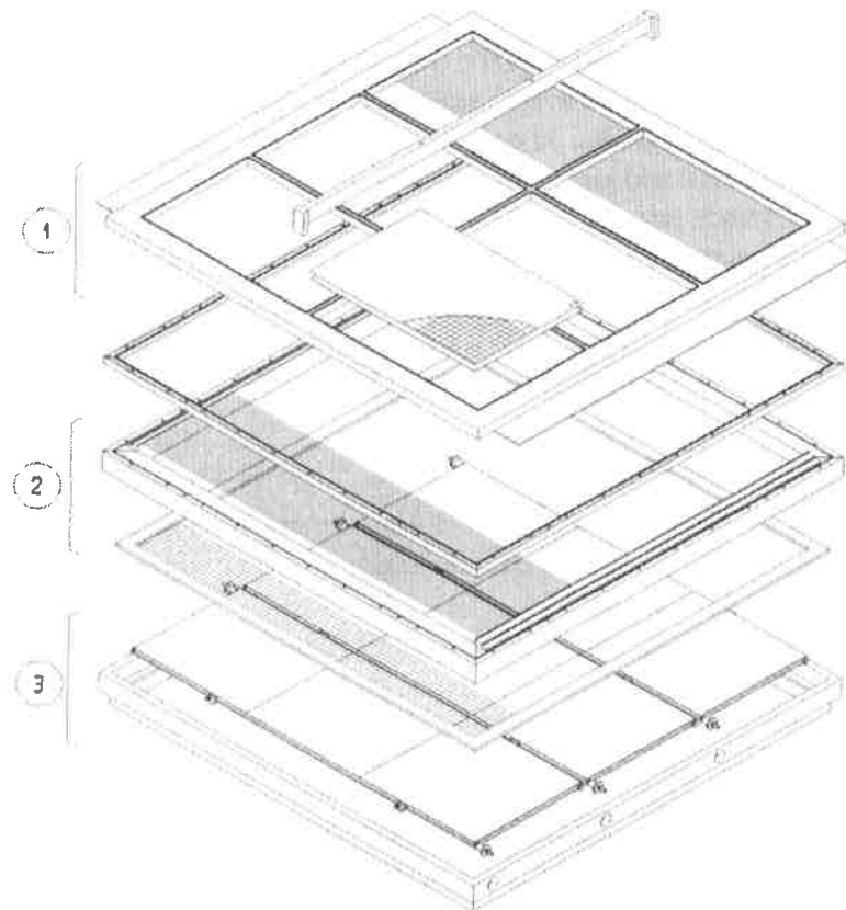
Figure 3.2: Axonometric view of a HMPID module. (1), (2), (3) are the elements described as Frame-1, Frame-2, Frame-3, respectively.
