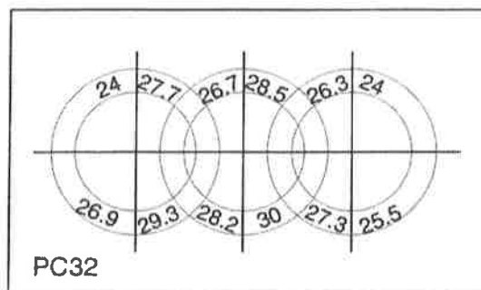
Figure 2.53: Evaluation of the uniformity of the chamber gain across PC32 in proto-2. The numbers correspond to the mean PH spectrum measured in 90^\circ sectors of the Cherenkov fiducial zones. HV = 2050 V.
