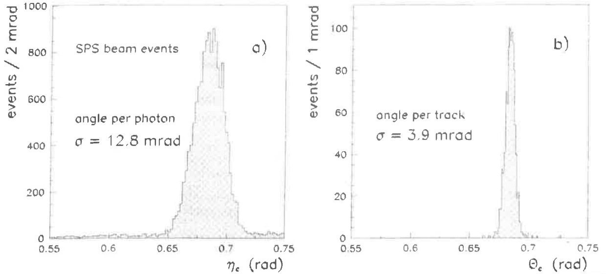
Figure 4.14: Photon angle distribution (a) and track Cherenkov angle distribution (b) for beam events at the SPS in data sample (1).
