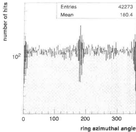
Figure 2.54: Azimuthal distribution of number of hits by 1^\circ bin along the Cherenkov fiducial zone. (3000 events, PC32, 2050 V).
