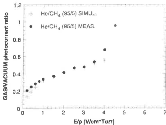
Figure 2.5: The ratio of the photocurrent from CsI, at 185 nm, in \text{He}/\text{CH}_4 (95/5) at 800 Torr, to that in vacuum (measured at the same absolute electric field) and the simulation results as a function of E/p at the photocathode surface.
