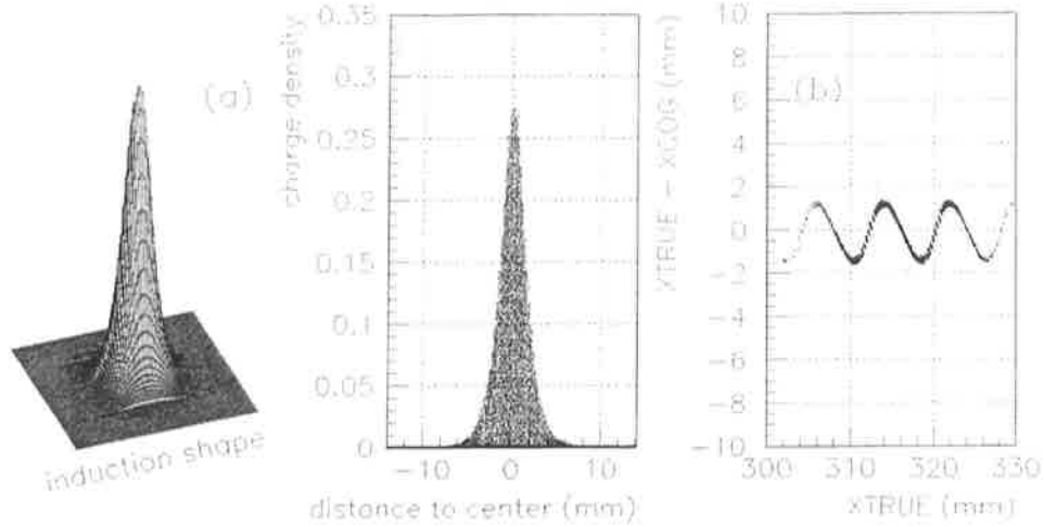
Figure 2.19: (a) Two-dimensional shape (left) and projection in one direction (right) of the charge distribution on the pad cathode. (b) Non linearity in the residuals distribution as a function of the true particle impact on 8 mm pads (the edges of the central pad are positioned at 312 and 320 mm).
