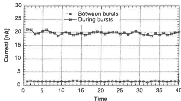
Figure 2.49: Sequence of chamber current values recorded between and during bursts of 10 000 particles. Each point is the mean of 40 bursts. HV = 2050 V, 10 000 particles/burst.
