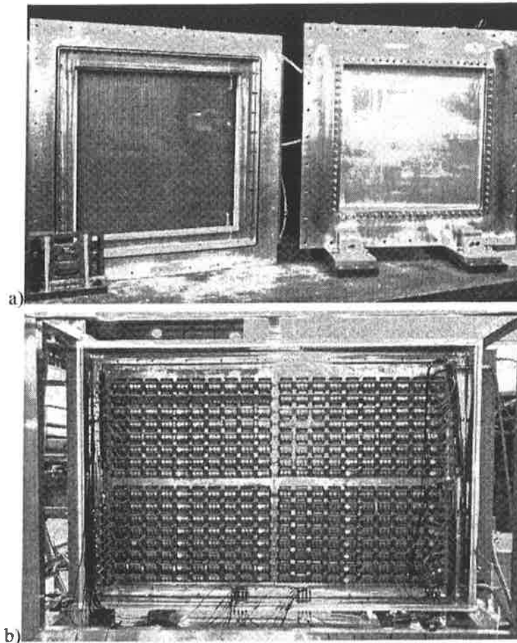
Figure 2.27: a) View of proto-1. On the left side, one sees the photodetector with a pad panel of 56 \times 60 pads and on the right side the radiator vessel enclosed by a quartz plate of 440 \times 460\ \text{mm}^2 . b) Proto-2 viewed from the pad panel side. The four independent pad panels instrumented with GASSIPLEX chips can be distinguished.
