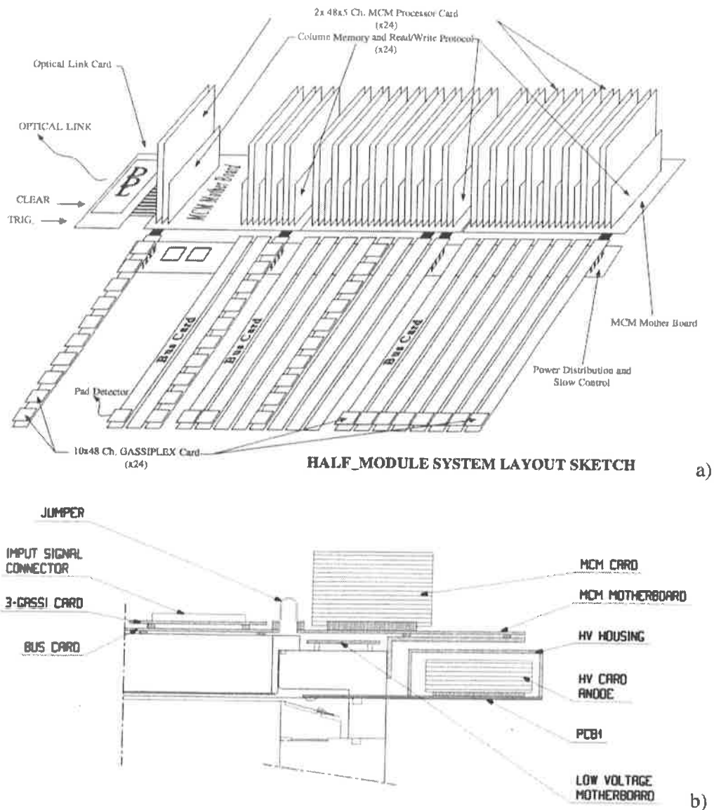
Figure 3.34: (a) Axonometric view of the electronics boards on the HMPID module. (b) mechanical fixation of the electronics boards on the module.
