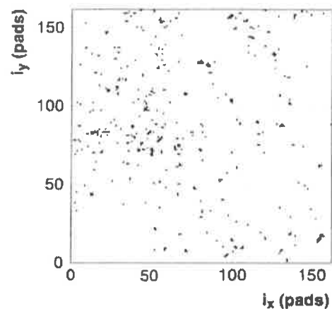
Figure 4.7: Same as Fig. 4.4, but for gammas only.
