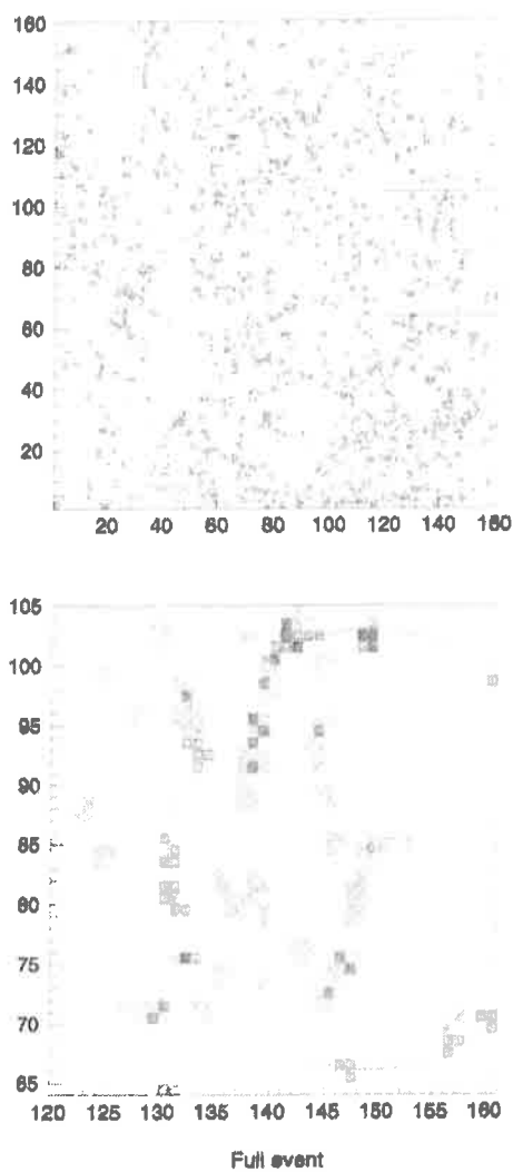
Figure 4.22: Top: hit map of one HMPID module in ALICE generated with the GALICE package for one Pb–Pb event. Bottom: zoom of the region enclosed by the box in the top map with the Cherenkov pattern (ring) associated to the Hough method.
