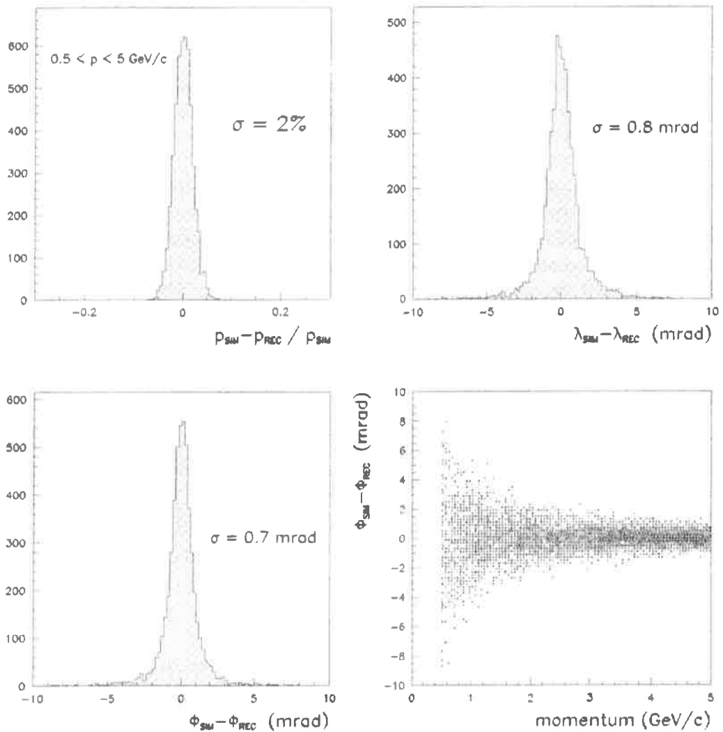
Figure 4.23: Residuals of simulated and reconstructed kinematic parameters.
