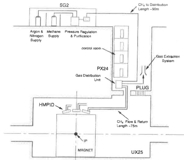
Figure 3.39: Schematic of the gas distribution system.
