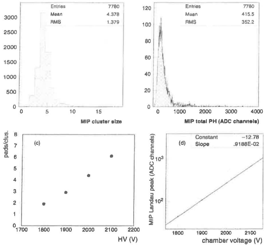
Figure 2.38: MIP studies with proto-2, PC31, CH 4 , empty radiator, 350 GeV/c pion. a) Cluster size distribution. b) Landau PH distribution at 2000 V. c) Primary cluster size as a function of HV. d) MIP Landau peak as a function of HV.
