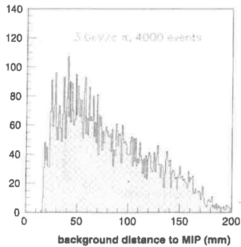
Figure 2.41: MIP studies with proto-1, PC24, 2050 V, CH 4 , empty radiator, 3 GeV/c pion. Distribution of the distances of secondary clusters to the impact of their primary MIP.
