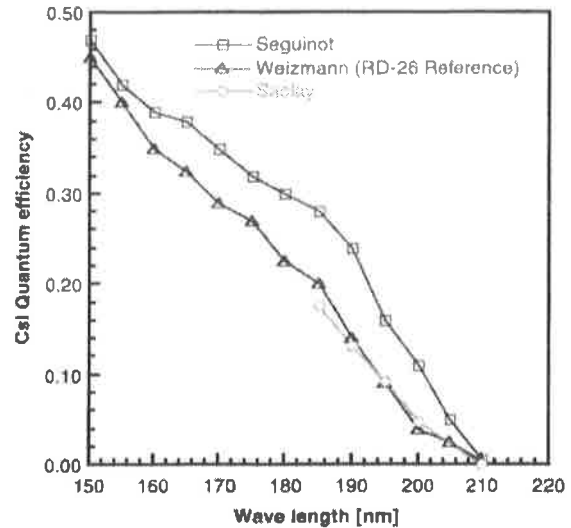
Figure 2.2: Measurements of the CsI QE as a function of wave length: a) Seguinot et al., best result from Ref. [2]; b) Weizmann, average curve [19]; c) Besson et al. [4]. Measurements a) and b) were made under vacuum.
