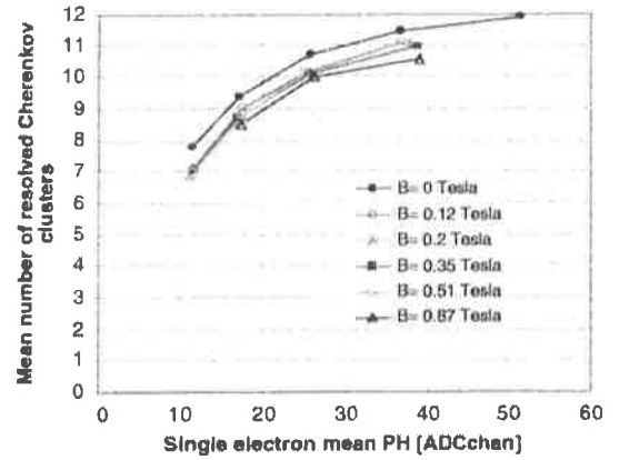
Figure 2.44: Measurement of the photoelectron yield ( N_{\text{res}}/\text{ring} ) of a CsI photocathode varying the chamber gain at different intensities of the magnetic field. Part of the drop respective to the no-field value originates from an increase of the common noise induced by the magnet operation. Experimental conditions: proto-1, PC24, CH 4 , 10 mm C 6 F 14 radiator, pion 350 GeV/c. One ADC channel corresponds to 0.17 fC.
