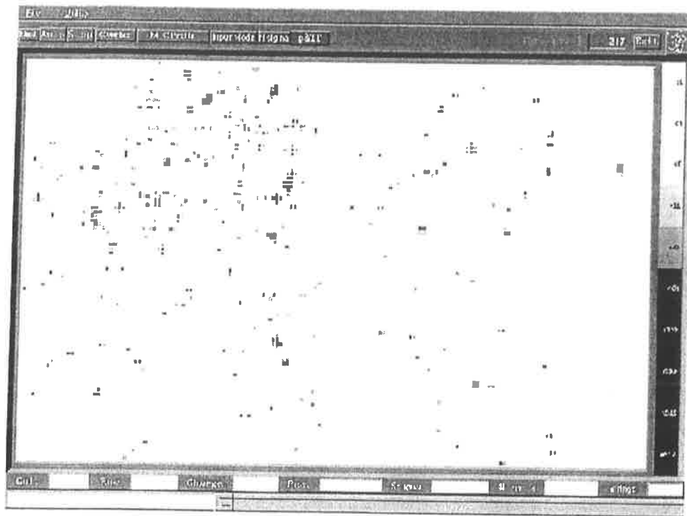
Figure 1.iv: Online screen display of an event recorded with the PROTO-2 module, using 350 \text{ GeV}/c \pi^- -Be interactions at the SPS. The colour code represents the charge collected per pad.
