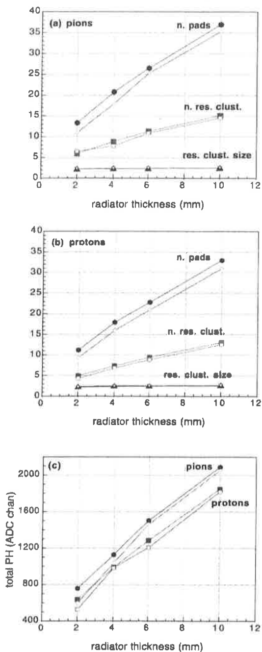
Figure 2.73: Radiator thickness scan in proto-1, PC24, 3 GeV/c PS beam test, chamber voltage 2250 V; full symbols: measurements; empty symbols: simulation. Number of pads, number of resolved clusters and resolved cluster size for pions (a) and protons (b) and total PH per event (c) as a function of the C_6F_{14} thickness.
