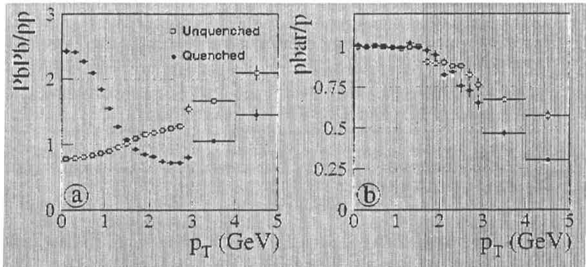
Figure 1.2: Expected influence of jet quenching on the ratio of proton p_t spectra between Pb–Pb and pp collisions (a) and on \bar{p}/p ratio in Pb–Pb collisions (b). The statistics corresponds to 10^7 pp and 5 \times 10^4 central Pb–Pb collisions.
