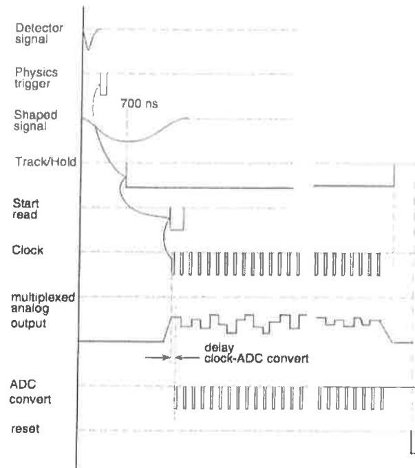
Figure 3.16: Time sequence of the control signals operating the multiplexed readout of GASSIPLEX-1.5.
