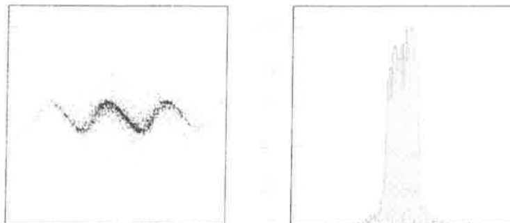
Figure 2.42: Smearing due to feedback photoelectrons of the residual distribution (compare to Fig. 2.19b).
