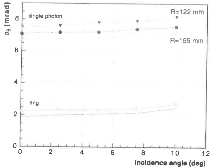
Figure 2.65: Angular resolution as a function of particle inclination at A_0 \sim 40 ADC channels; circles ( R = 155 mm) and triangles ( R = 122 mm): measurements; crosses: ( R = 155 mm) simulation; SPS beam-test ( 350 \text{ GeV}/c \pi ), R = 122 mm: PC30 and GAP = 80 mm, R = 155 mm: PC32 and GAP = 103 mm.
