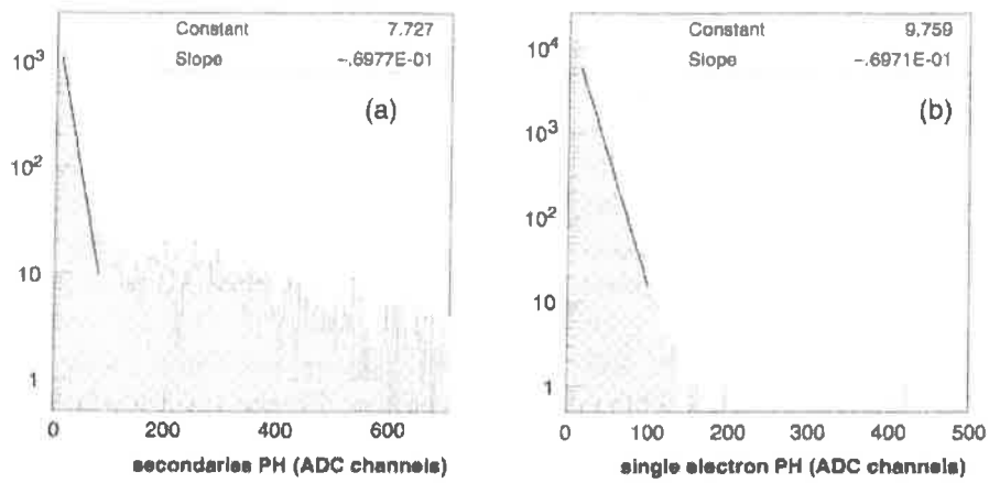
Figure 2.40: MIP studies with proto-2, PC31, 2000 V, CH 4 , empty radiator, 350 GeV/c pion. a) PH spectrum of secondary clusters associated to a MIP cluster. b) For comparison, PH spectrum of single Cherenkov photoelectrons at the same voltage. One ADC channel corresponds to 0.17 fC.
