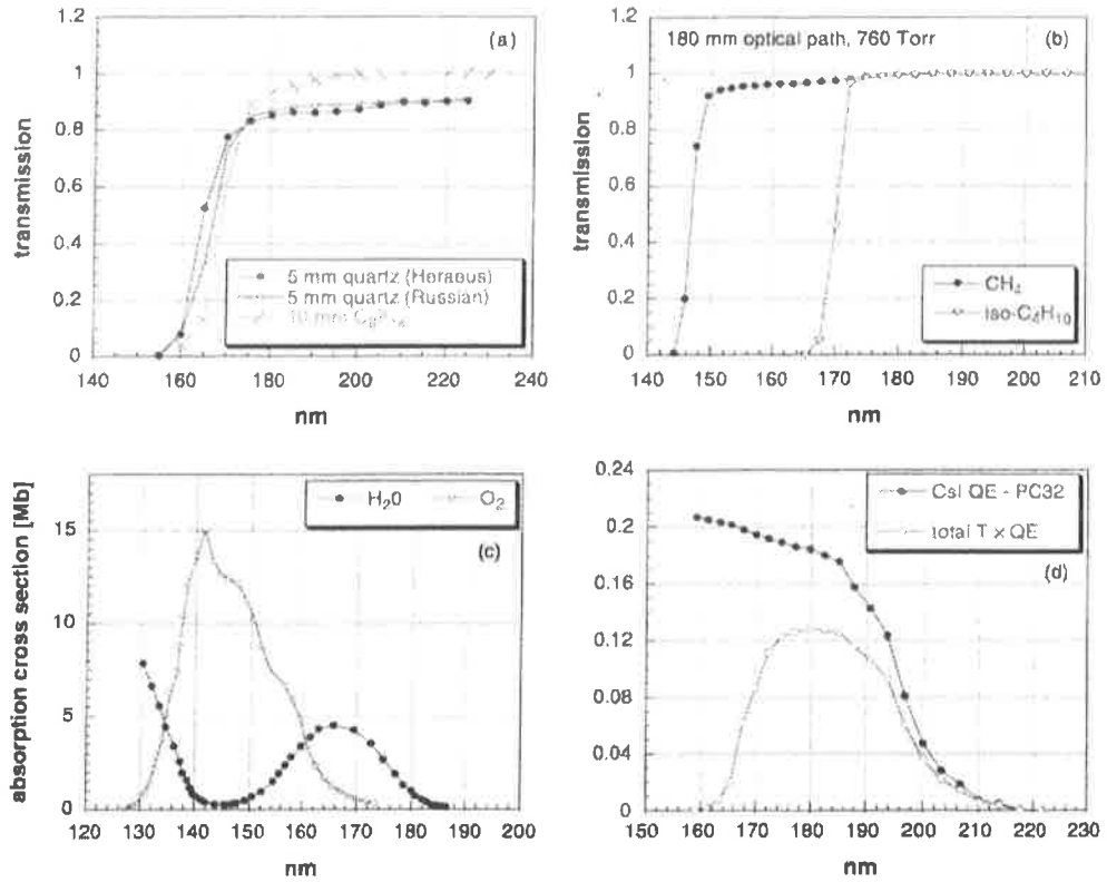
Figure 2.24: (a) Measured UV transmission of 10 mm C 6 F 14 and 5 mm quartz plates (not corrected for reflection losses). (b) UV transmission of CH 4 and iC 4 H 10 , calculated from [49] and [50] respectively, for a photon path of 180 mm equivalent to a distance travelled in a proximity gap of 103 mm by Cherenkov photons emitted in C 6 F 14 by \beta = 1 particles. (c) UV absorption cross section of oxygen [51] and water [52]. (d) PC32 QE evaluated from simulation (Section 2.4.2) and the convolution with the total media transmission.
