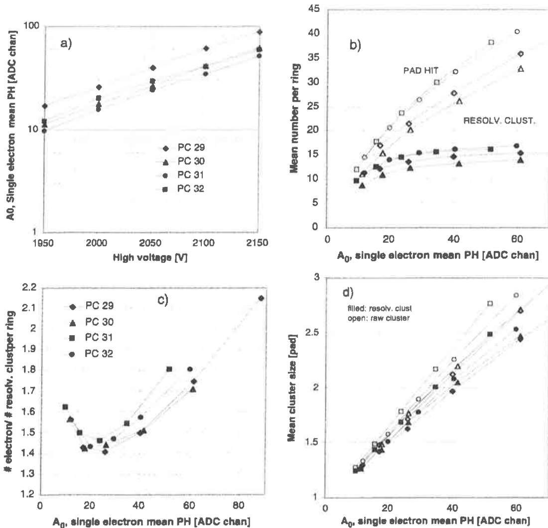
Figure 2.59: Compared performance of the four photocathodes mounted on proto-2. Operating conditions: \text{CH}_4 , 10 mm \text{C}_6\text{F}_{14} , pion 350 GeV/c. One ADC channel corresponds to 0.17 fC. a) Mean single-electron PH (or chamber gain) as a function of high voltage measured at the centre of each of the four PCs. As a function of the single-electron mean PH: b) Mean N_{\text{res}} and N_{\text{pad}} per ring. c) Ratio N_{\text{tot}}/N_{\text{res}} (feedback photon fraction). d) Mean resolved cluster size.
