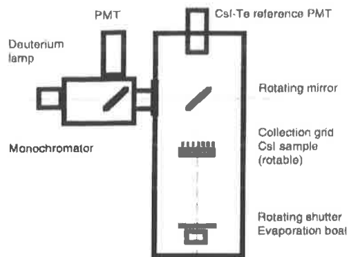
Figure 2.1: Scheme of the set-up used to measure the QE of CsI evaporated on small samples. After coating, the sample is rotated by 180^\circ , under vacuum, to be illuminated from the top by the UV collimated beam.
