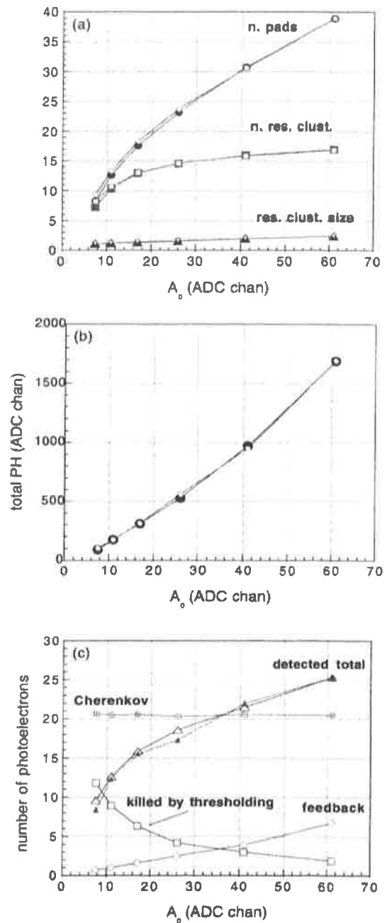
Figure 2.74: Chamber gain scan in proto-2, PC32, 350 GeV/c \pi SPS beam test; full symbols: measurements; empty symbols: simulation. Number of pads, number of resolved clusters and resolved cluster size (a) and (b) and total PH per event; in (c) the measured total number of detected photoelectrons estimated is compared to the same quantity obtained from the simulation, with an evaluation of the single contributions (detected total = Cherenkov+feedback-killed by thresholding).
