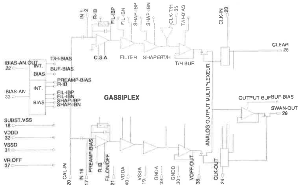
Figure 3.15: Schematics of the functional blocks composing GASSIPLEX-1.5.
