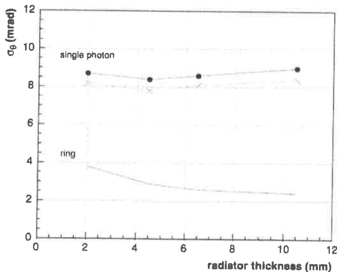
Figure 2.66: Angular resolution as a function of radiator thickness at R = 104 mm; circles: measurements; crosses: simulation; PS beam-test ( 3 \text{ GeV}/c \pi ), PC24.
