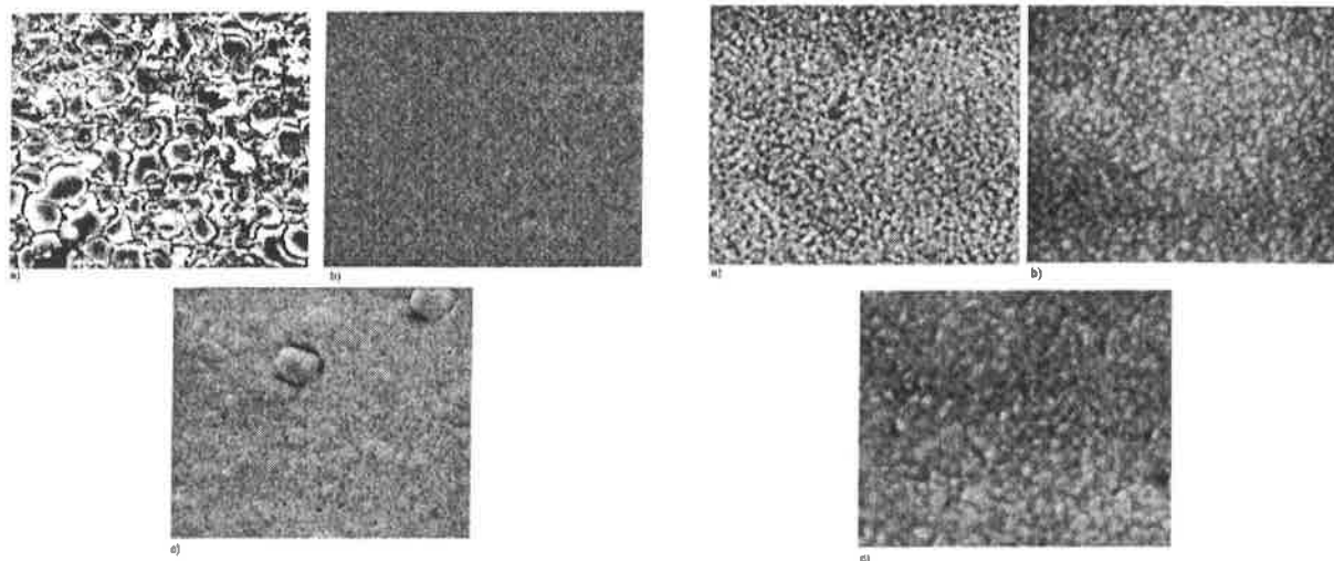
Figure 2.12: SEM images: \times 2500 . CsI layers, 500 nm thick, deposited on various substrates: a) G10/Cu/Au, b) glass/Ni/Au, c) G10/Cu/Ni/Au.
