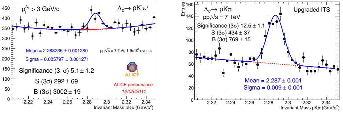
Figure 2.36: \Lambda_c \rightarrow pK^-\pi^+ candidates invariant mass distribution for p_t > 3 \text{ GeV}/c in pp collisions at 7 TeV ( 1.9 \times 10^8 events). Left: pp collision data. Right: Hybrid simulation with the ITS upgrade configuration. The sample statistics in the simulation is the same as in the data, while the selection cuts were optimized specifically for the upgrade scenario.
