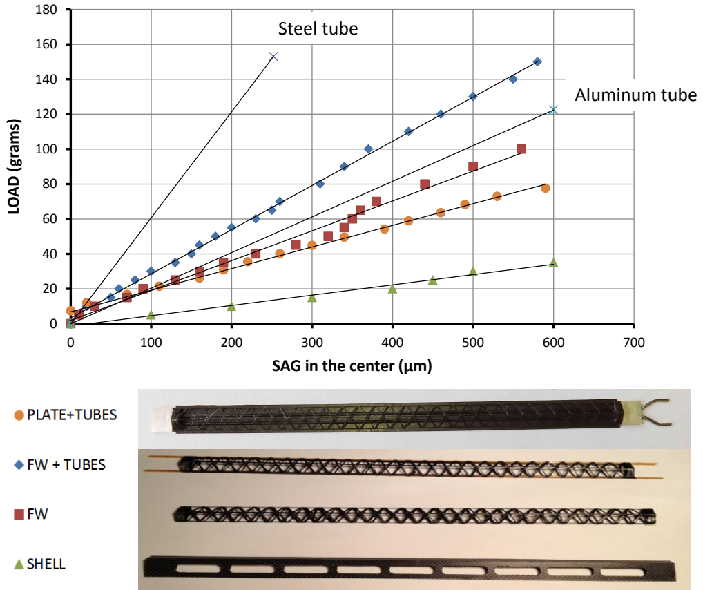
Figure 5.12: Bending test results performed on the four prototype structures. A tube made in aluminum and one in steel with an equivalent section have been added to the plot as reference.
