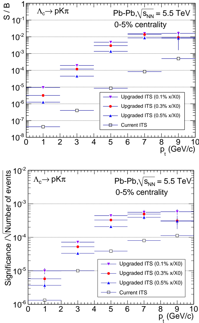
Figure 2.37: \Lambda_c \rightarrow \rho K \pi in central Pb–Pb collisions at \sqrt{s_{NN}} = 5.5 TeV: signal-to-background ratio (upper panel) and significance per event (lower panel) for current and upgraded ITS. For the upgrade, three different scenarios are considered: the baseline configuration is labelled “0.3%”; the cases labelled “0.1%” and “0.5%” represent variations of the layer thickness only (with respect to the baseline configuration), for the innermost two layers to 0.1% of radiation length and for all layers to 0.5% of radiation length, respectively.
