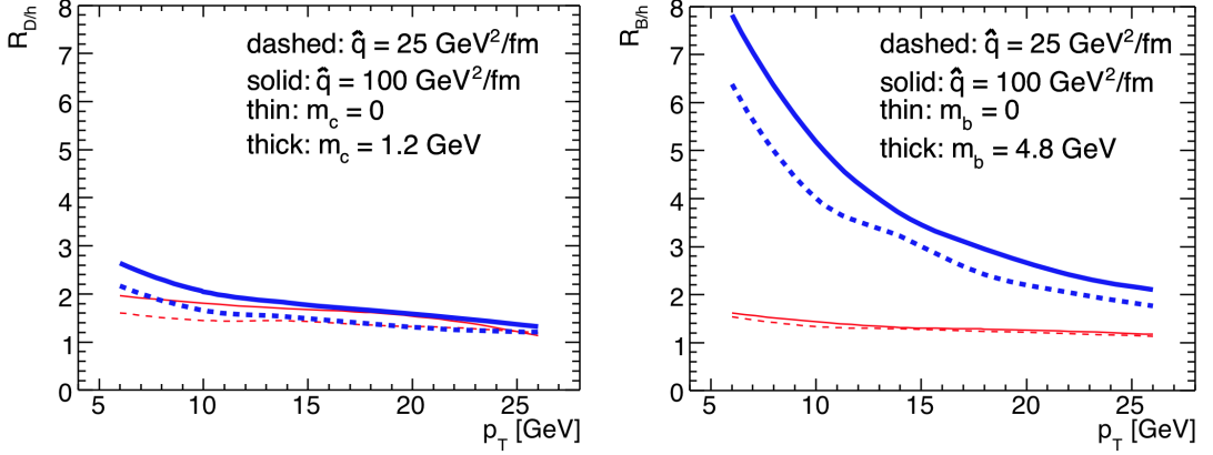
Figure 2.11: Heavy-to-light R_{AA} ratios as predicted by radiative energy loss (ASW) [47]. Left: R_{AA}^D/R_{AA}^h . Right: R_{AA}^B/R_{AA}^h .
