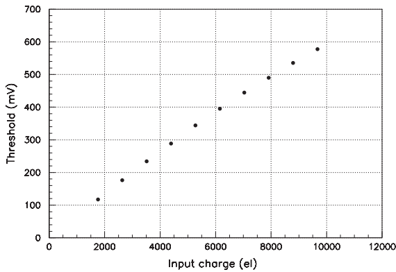
Fig. 7. Linearity of the amplifier and shaper part of the RX64 chip.
