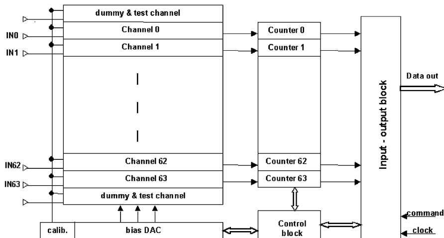
Fig. 5. Block diagram of the RX64 chip.
