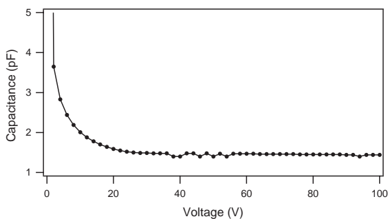
Fig. 2. C - V curve for a group of four contiguous strips.
