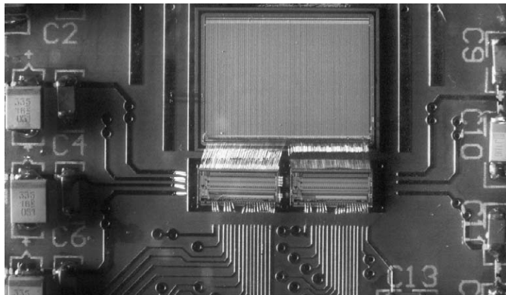
Fig. 6. Photograph of the board with 132-strip detector and two RX64 ASICs.
