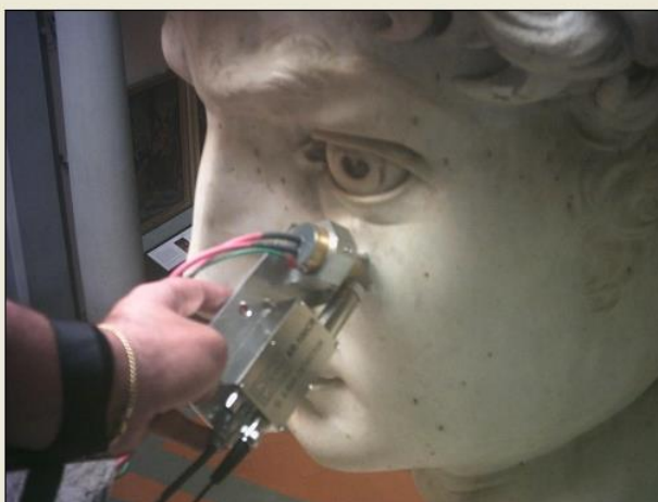
XR-100CR shown taking an x-ray fluorescence spectrum of David.
