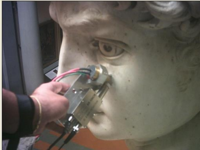
XR-100CR shown taking an x-ray fluorescence spectrum of David.
