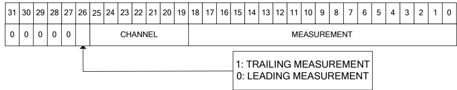
Fig. 6.2: Output Buffer: the TDC Header
